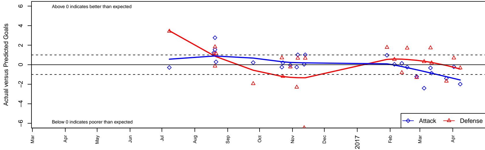
ISC Gunners Select G02 Dots are actual minus expected GF (blue circles) and GA (red triangles). Blue line is smoothed change in attack strength. Red is smoothed change in defense strength.
